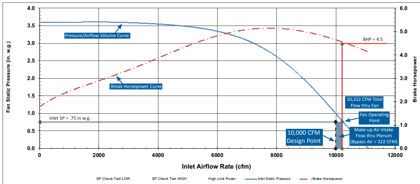
Example Selection: 10,000 CFM Exhaust at .75" w.g. Inlet Static Pressure
